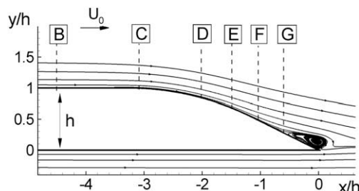
Fig. 13. Schematic of the hydrofoil and mean flow streamlines from IDDES. Letters denote positions of sections, where experimental data of Blake, 1975 and full-LES of Wang and Moin (2002) are available (B: x/h = -4.5 ; C: -3.125 ; D: -2.125 ; E: -1.625 ; F: -1.125 ; G: -0.625 ).
